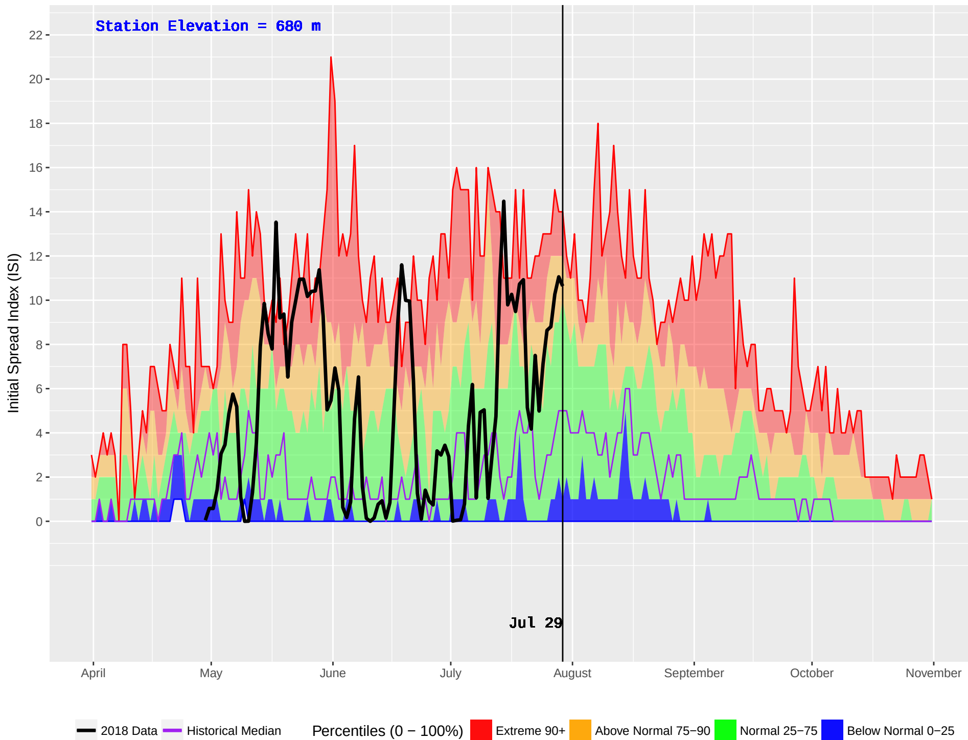
REVELSTOKE (363) : Historical (1995–2016) and Current (2018) Daily Initial Spread Index (ISI)
