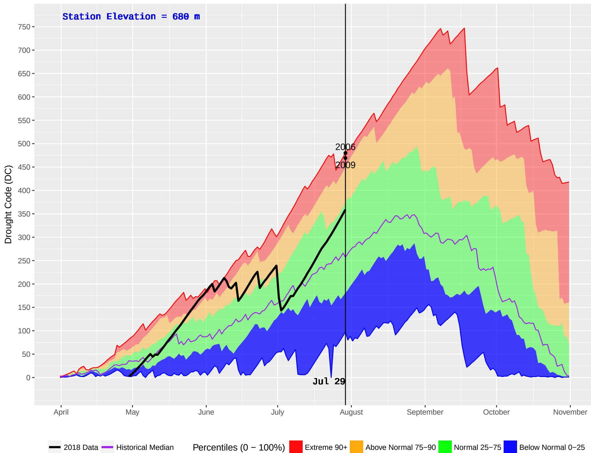
REVELSTOKE (363) : Historical (1995–2016) and Current (2018) Daily Drought Code (DC)
